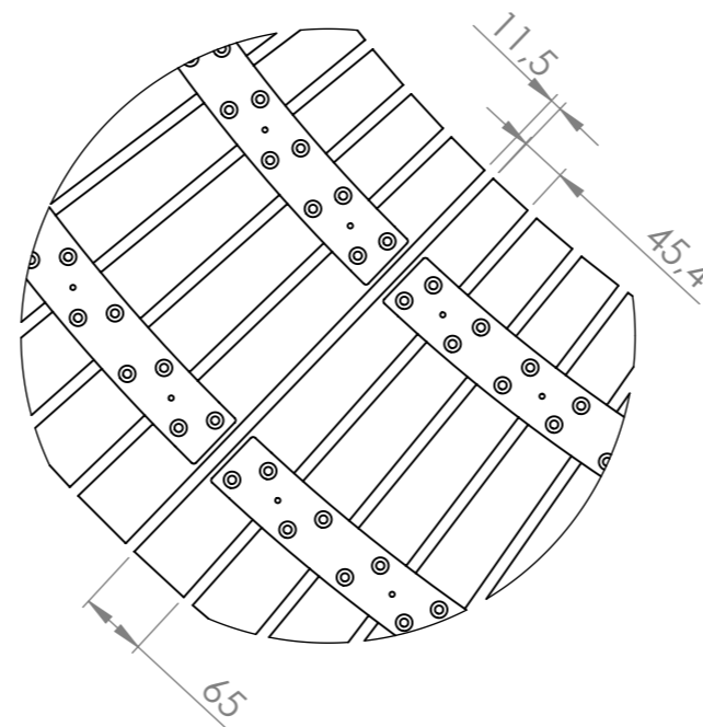
DETAIL A
